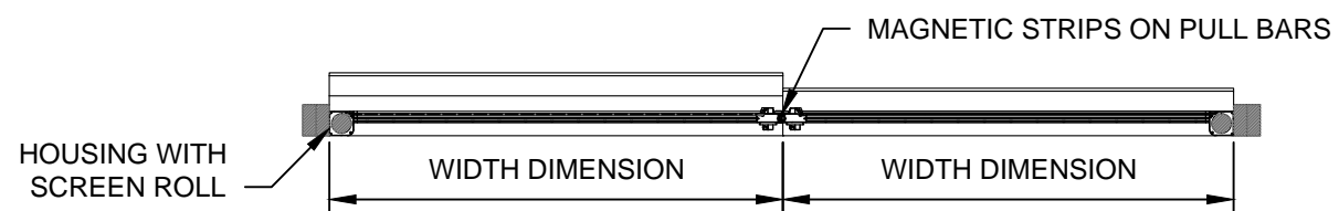
VISTA VIEW SPLIT LEVEL SECTION
