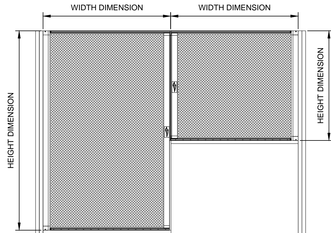
VISTA VIEW SPLIT LEVEL TYPICAL ELEVATION
