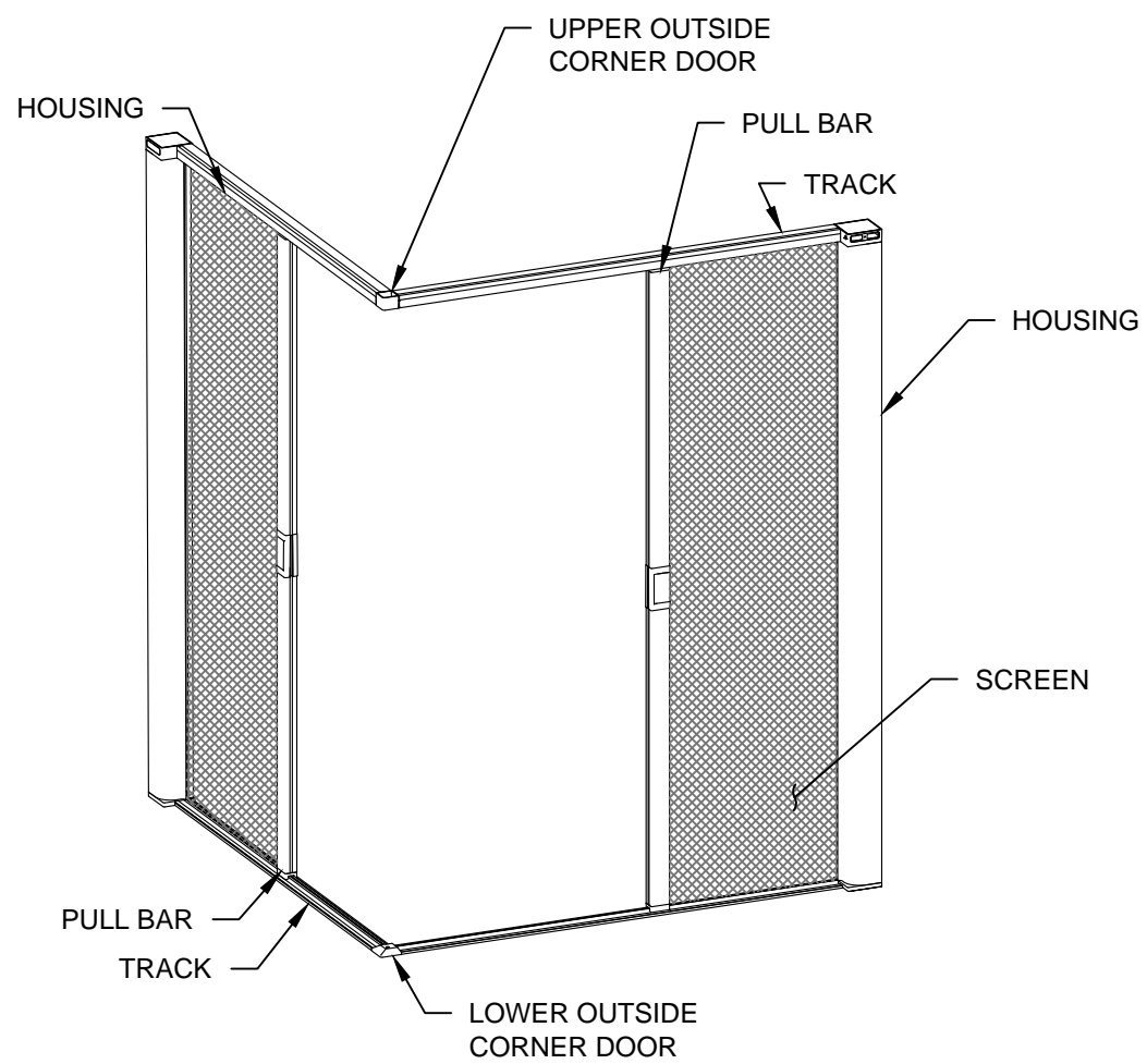
HORIZON CORNER UNIT EXTERNAL
