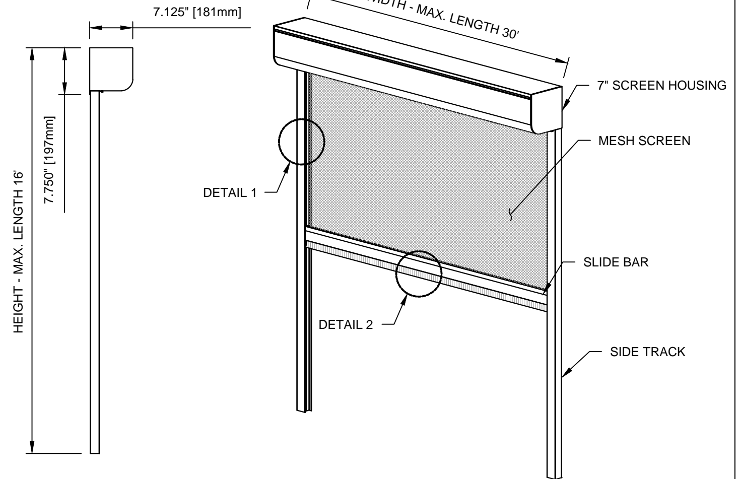
7" STANDARD SCREEN ASSEMBLY SCALE: 3/4" = 1'-0"
