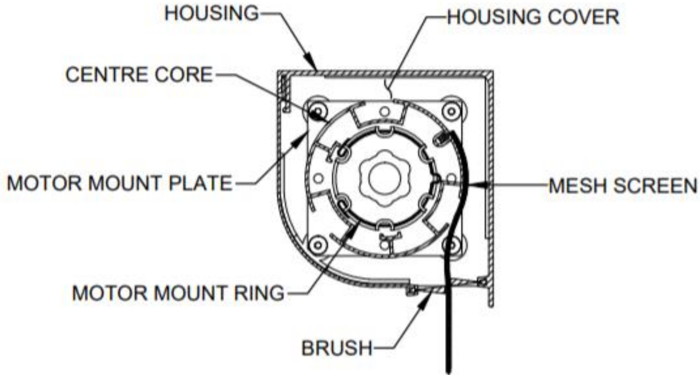
SECTION VIEW A Motor End
