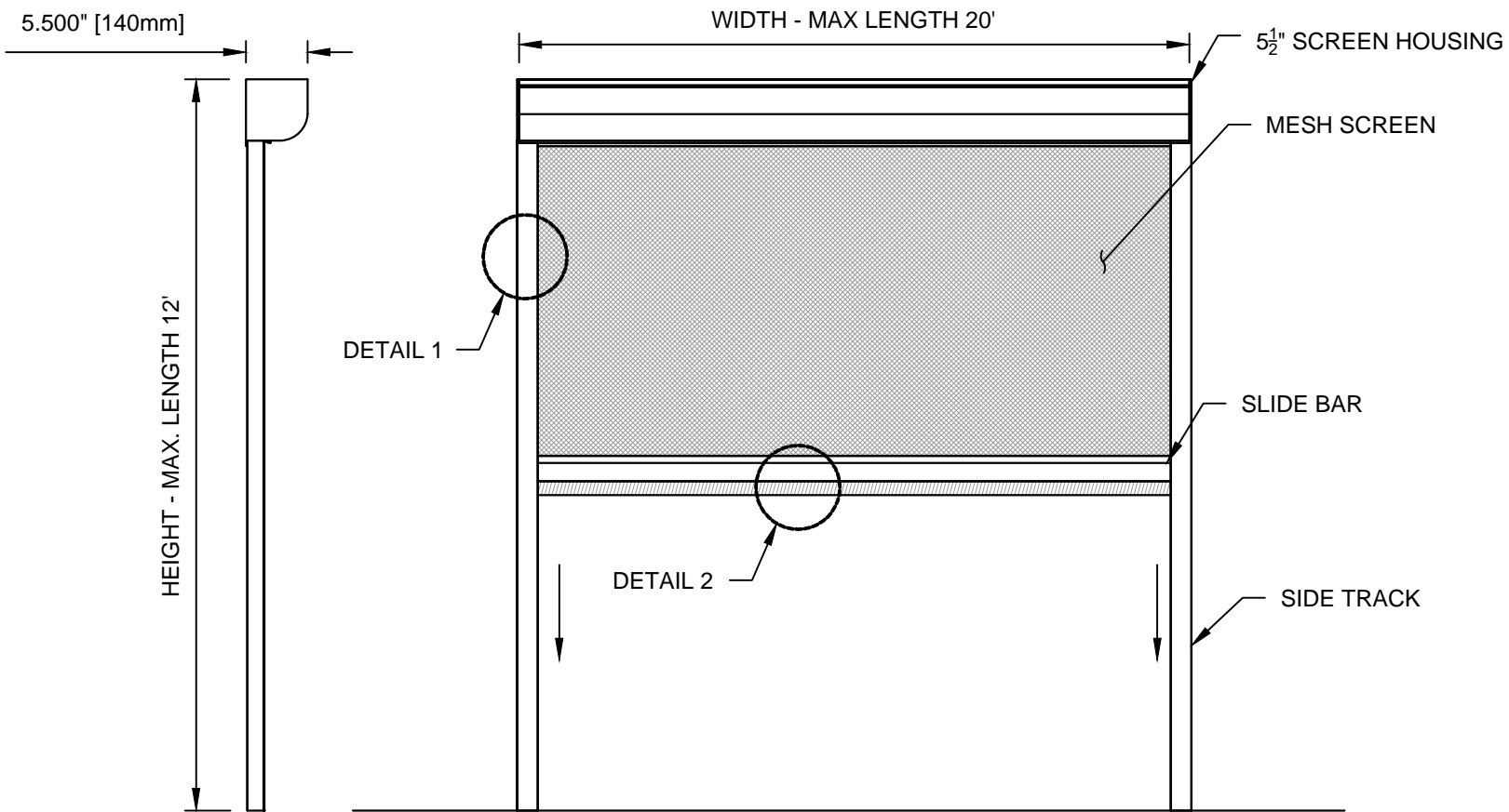
5 1/2" STANDARD SCREEN ASSEMBLY SCALE: 3/4" = 1'-0"
