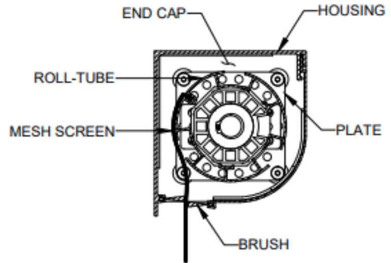
SECTION VIEW B
