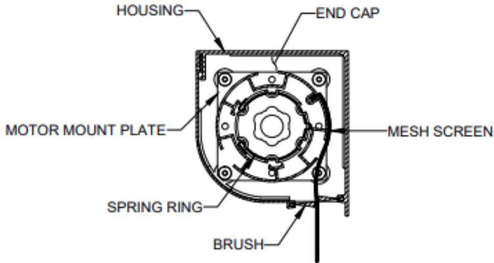
SECTION VIEW A
