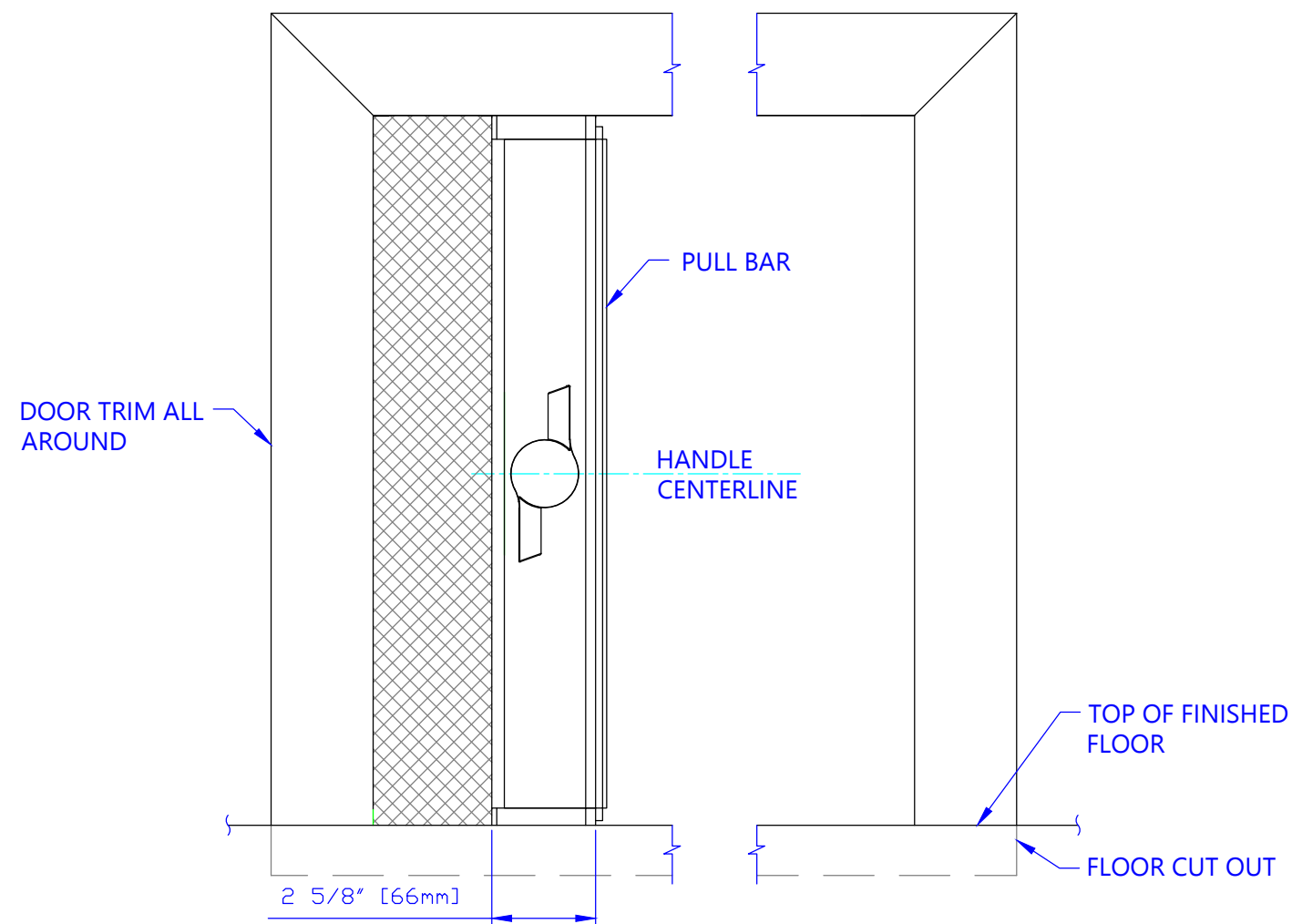
ELEVATION - FRONT VIEW
