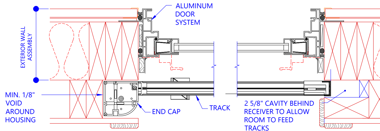
PLAN - SECTION VIEW
