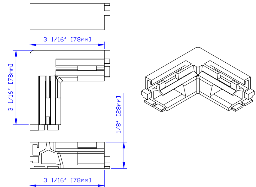
INTERNAL CORNER LATCH
