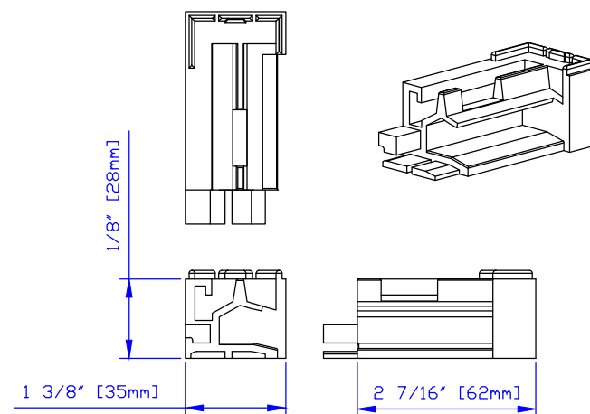
SINGLE LATCH
