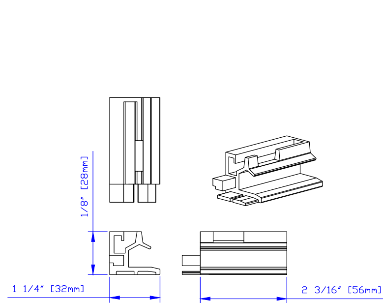
DOUBLE LATCH A
