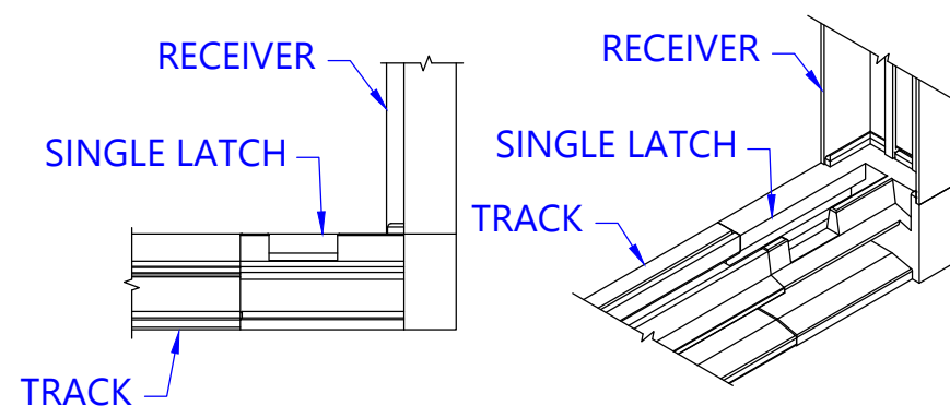
SINGLE LATCH CONNECTION
