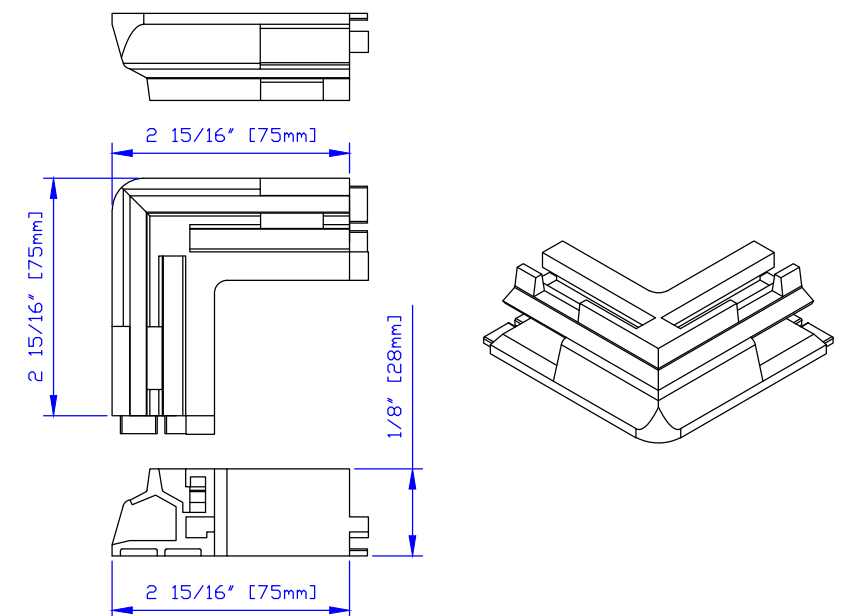
EXTERNAL CORNER LATCH
