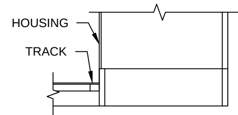
FRONT ASSEMBLY VIEW
