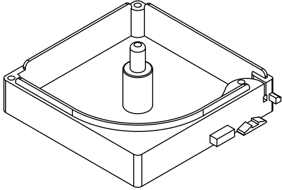
ISOMETRIC VIEW - BOTTOM LEFT
