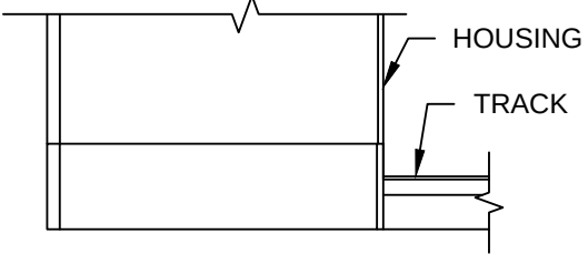
BACK ASSEMBLY VIEW
