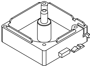
ISOMETRIC VIEW - BOTTOM LEFT
