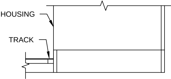
BACK ASSEMBLY VIEW
