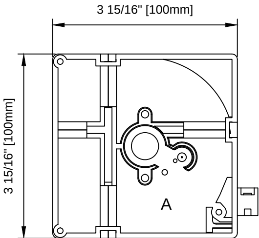
UNDERSIDE VIEW
