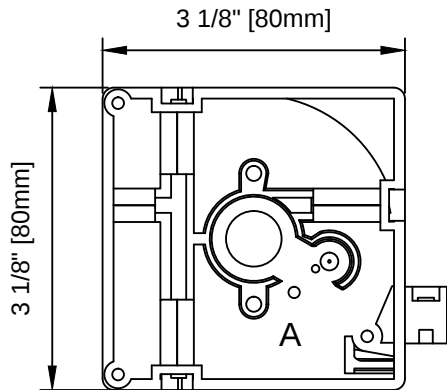
UNDERSIDE VIEW
