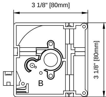
UNDERSIDE VIEW
