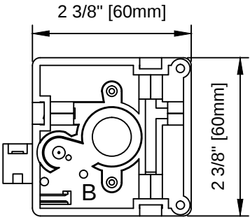
UNDERSIDE VIEW
