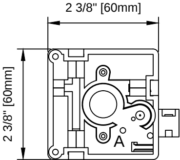
UNDERSIDE VIEW
