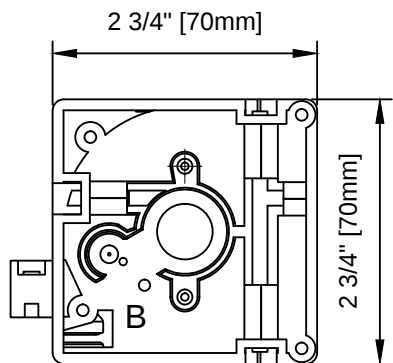
UNDERSIDE VIEW
